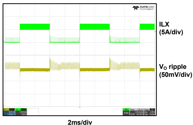
Load Transient 0A to 6A
