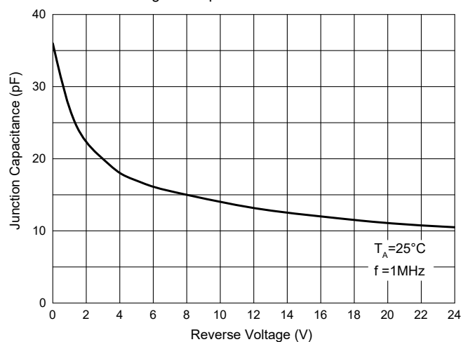
Fig. 3 - Capacitance Characteristics
