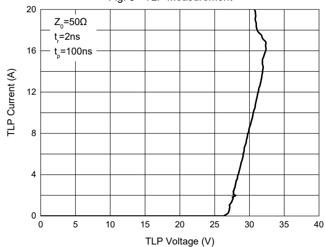
Fig. 5 - TLP Measurement
