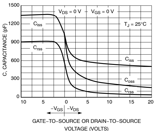
Figure 7. Capacitance Variation
