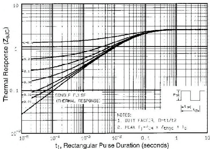
Fig. 10 - Maximum Effective Transient Thermal Impedance, Junction-to-Case
