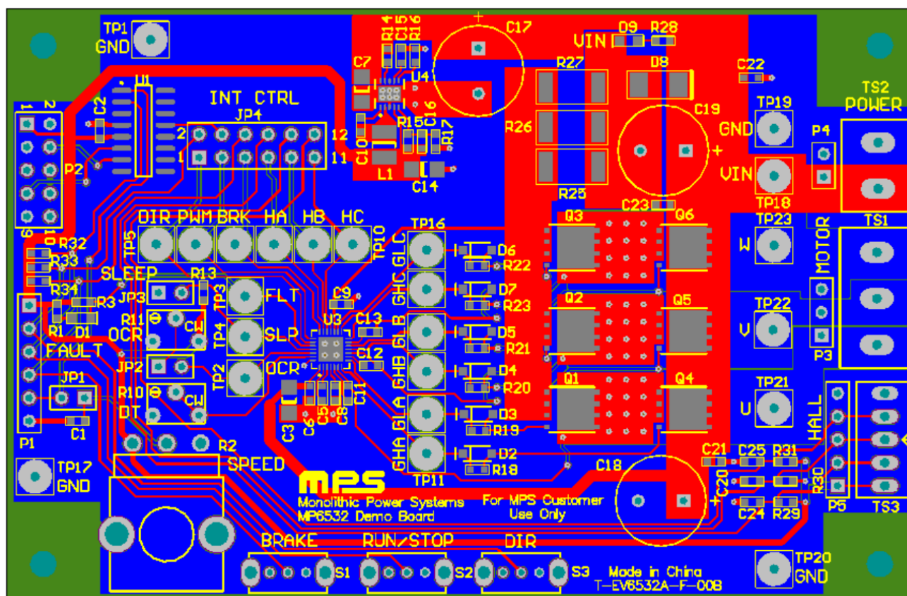
Figure 7: Recommended Layout
