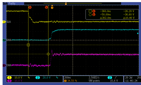
Figure 2: Dead Time
