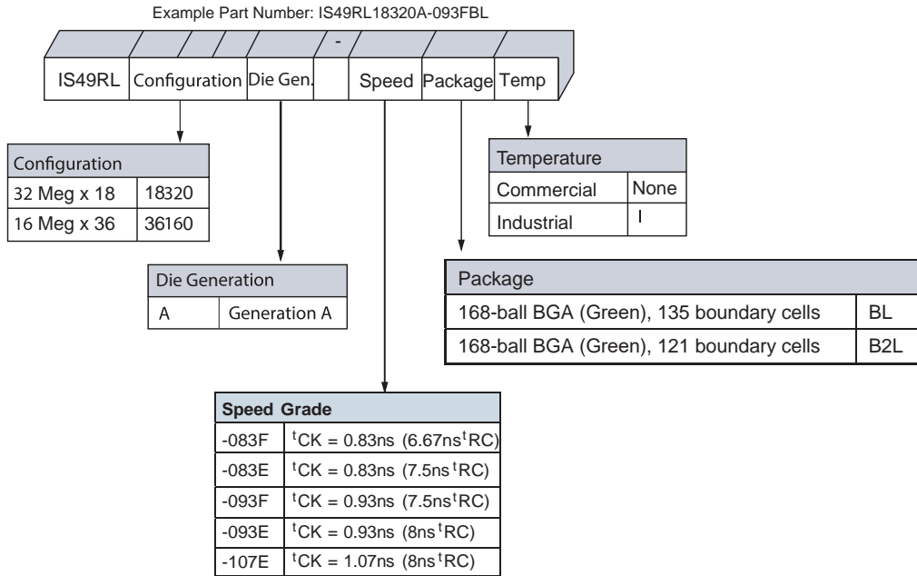
Figure 1: 576Mb RLD RAM ® 3 Part Numbers
