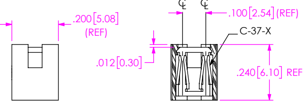
SECTION "A"-"A" SCALE 2.5 : 1
