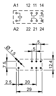
Copper side view Pin length 5.2 mm for PCB or sockets
