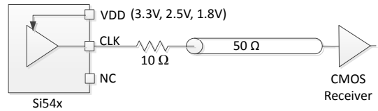
Single CMOS Termination
