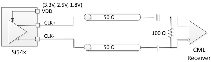
CML Termination without VCM
