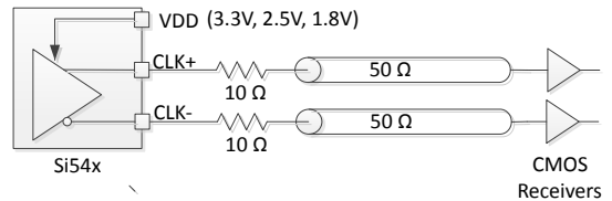
Dual CMOS Termination
