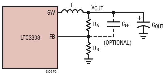
Figure 1. Feedback Resistor Network for the LTC3303 Adjustable Version
