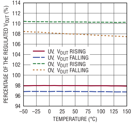
UV, OV PGOOD Thresholds vs Temperature
