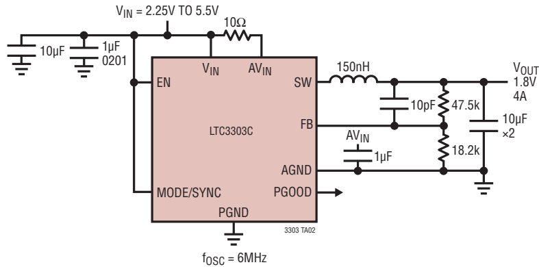
6MHz, V_{FB} Resistor Programmed, 1.8V, 4A, Burst Mode Operation
