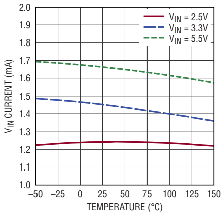
VIN Quiescent Current All Modes, Not Sleeping
