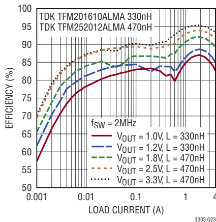
Efficiency, V_{IN} = 5.0V , Burst Mode Operation
