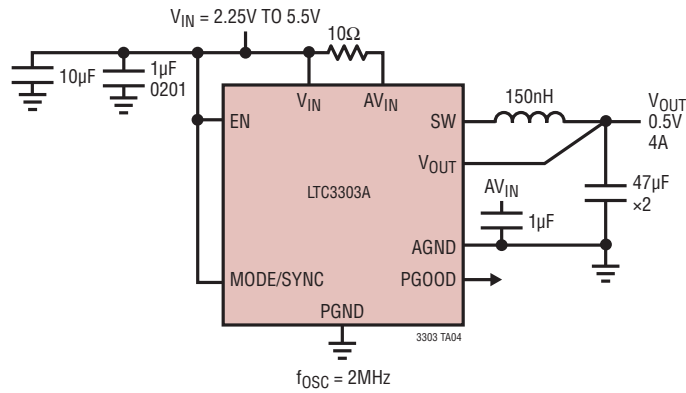
Fixed V_{OUT} , 0.5V, 4A, Burst Mode Operation
