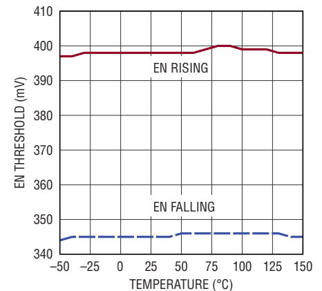
EN Threshold vs Temperature
