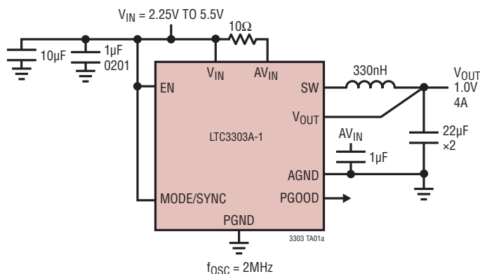
High Efficiency, 2MHz, 1V, 4A Step-Down Converter
