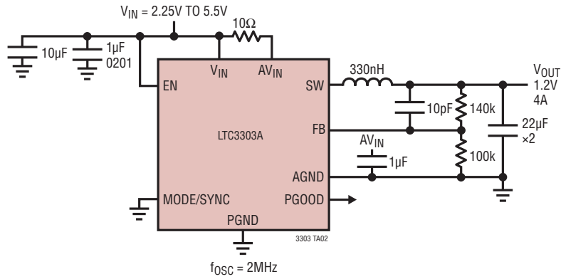
2MHz, V_{FB} Resistor Programmed, 1.2V, 4A, Forced Continuous Mode
