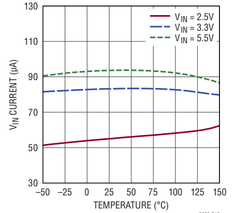
VIN Quiescent Current, Burst Mode Operation, Sleeping
