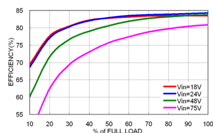
MPP03-48S05WA Efficiency vs. Output Load
