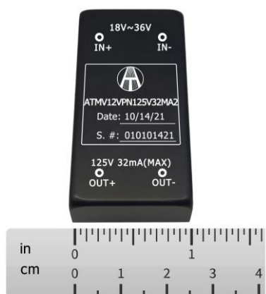
Figure 1. Top View of ATMV12VPN125V32MA2
