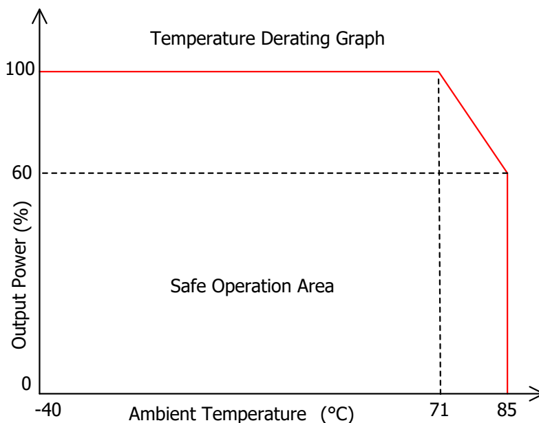
Figure 5. Derating Curve
