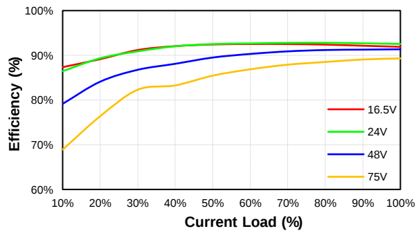
CHB500W-48S48 Eff Vs Io @25 Deg. C
