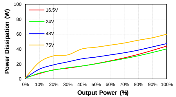
CHB500W-48S48 Pd Vs Po @25 Deg. C
