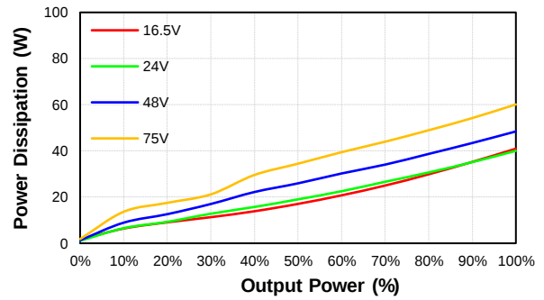
CHB500W-48S24 Pd Vs Po @25 Deg. C
