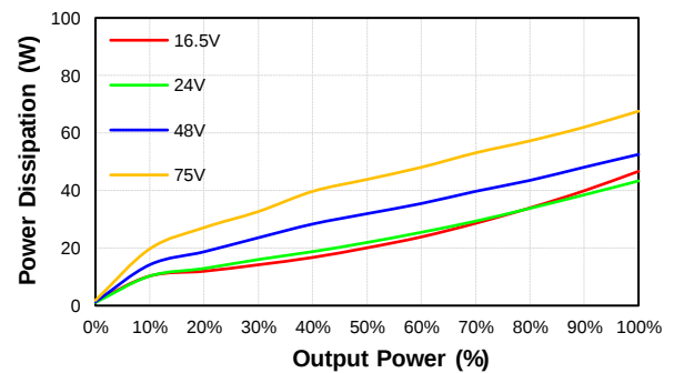
CHB500W-48S28 Pd Vs Po @25 Deg. C
