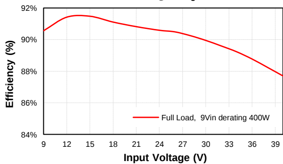
CHB500W-24S24 Eff Vs Io @25 Deg. C
