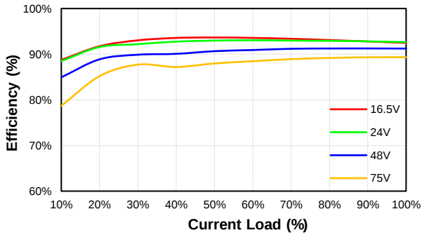
CHB500W-48S24 Eff Vs Io @25 Deg. C
