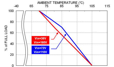
RCD15-110 Derating Curve
