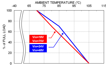
RCD15-48 Derating Curve
