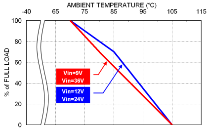
RCD15-24 Derating Curve
