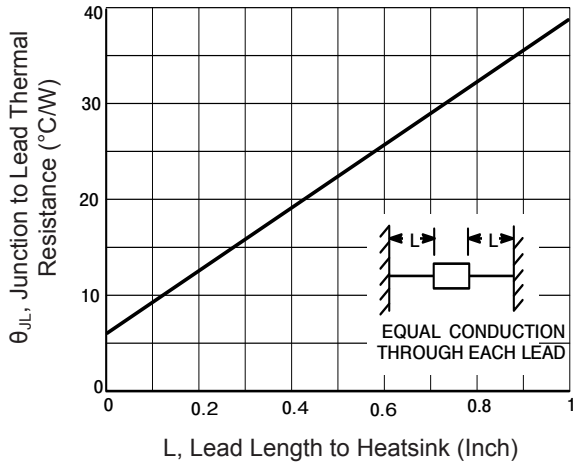
Figure 1. Typical Thermal Resistance
