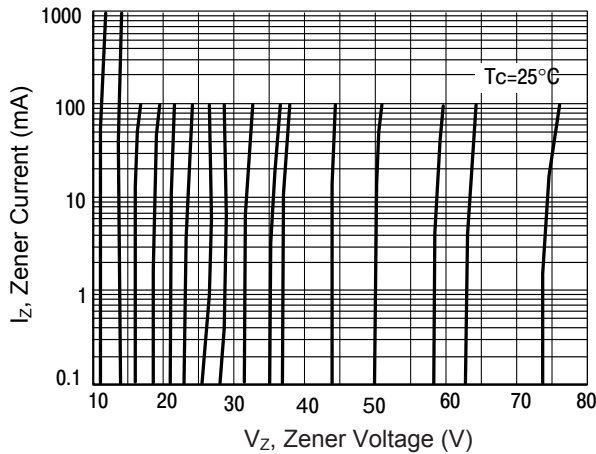
Figure 7. Zener Voltage vs. Zener Current V Z =11 thru 75 Volts
