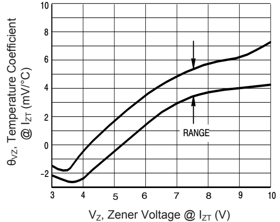
Figure 2. Temperature Coefficient-Range for Units 3 to 10 Volts
