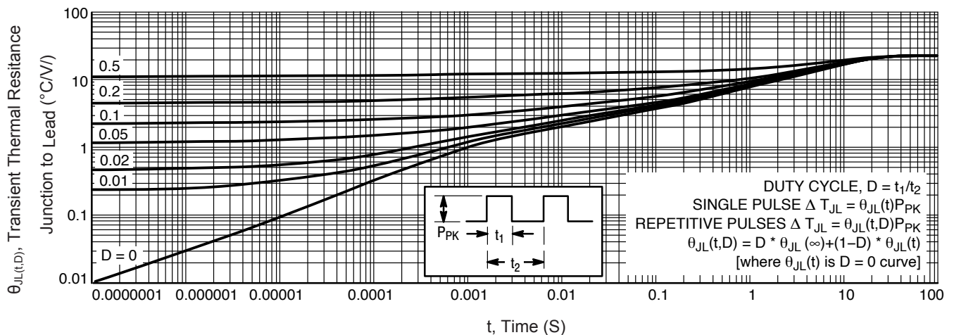
Figure 9. Typical Thermal Response L, Lead Length=3/8 Inch
