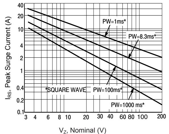
Figure 4. Maximum Non-Repetitive Surge Current vs. Nominal Zener Voltage (See Note 4)
