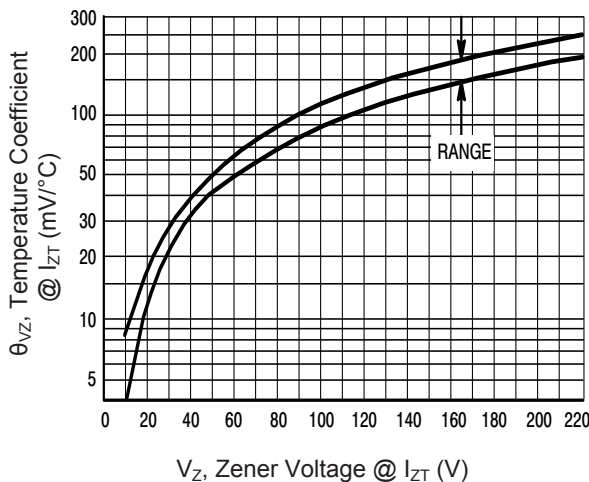
Figure 3. Temperature Coefficient-Range for Units 10 to 220 Volts
