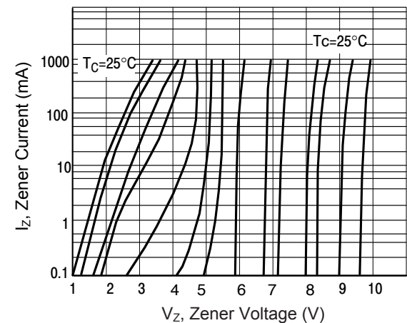
Figure 6. Zener Voltage vs. Zener Current V_Z = 3.3 thru 10Volts
