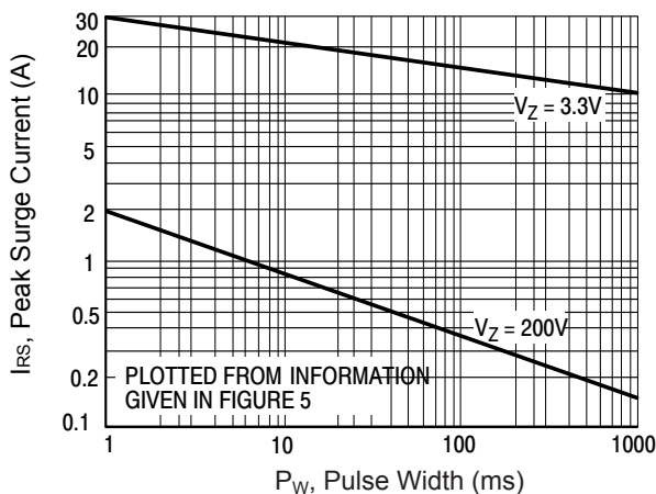
Figure 5. Peak Surge Current vs. Pulse Width (See Note 4)
