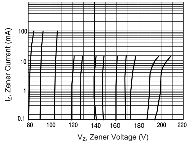
Figure 8. Zener Voltage vs. Zener Current V Z =82 thru 200 Volts
