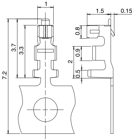
●DF13G
