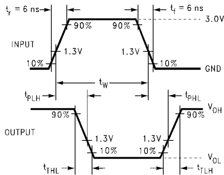
Figure 6. AC Waveforms
