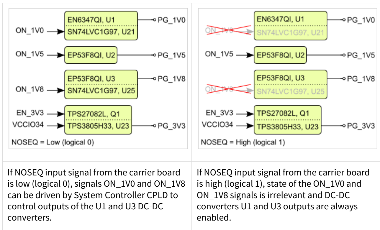
Figure 4: Power sequencing.
