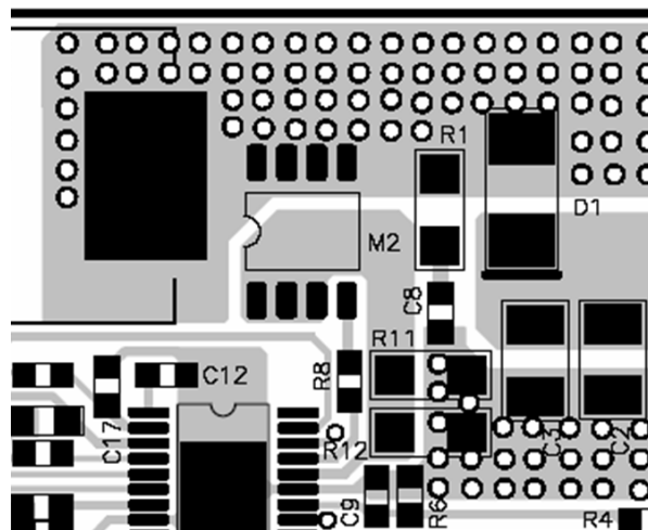
Figure 6—Layout Consideration
