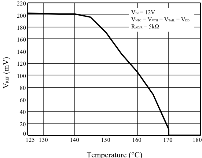
Figure 30 Thermal Rolloff
