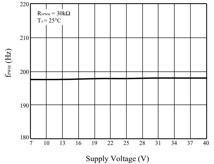
Figure 18 f_{PWM} vs. Supply Voltage (Internal PWM)
