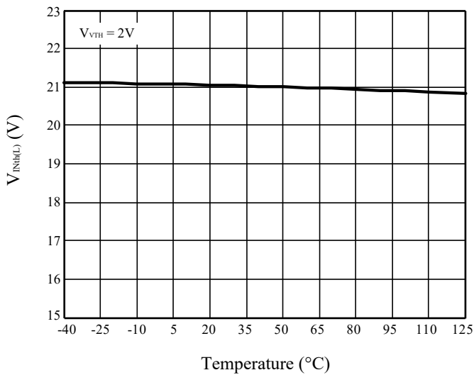
Figure 19 V_{INth(L)} vs. Temperature
