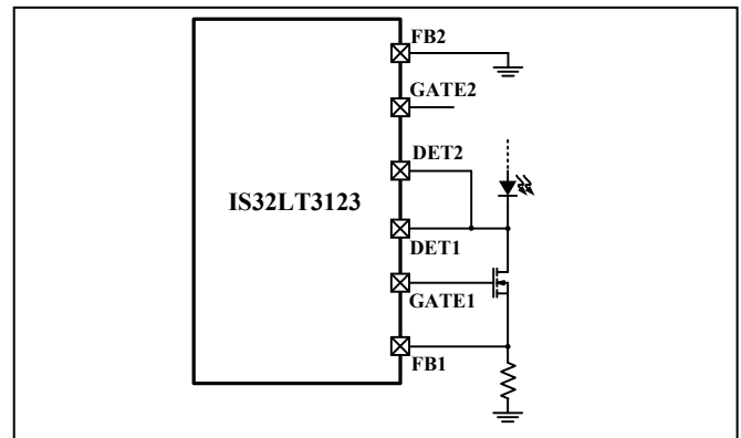
Figure 32 Unused Channel (CH1 Used and CH2 Unused)
