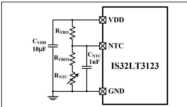
Figure 34 R_{TRO1} Slows Down Slew Rate
