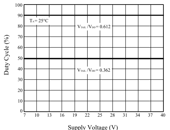
Figure 16 Duty Cycle vs. Supply Voltage (Internal PWM)
