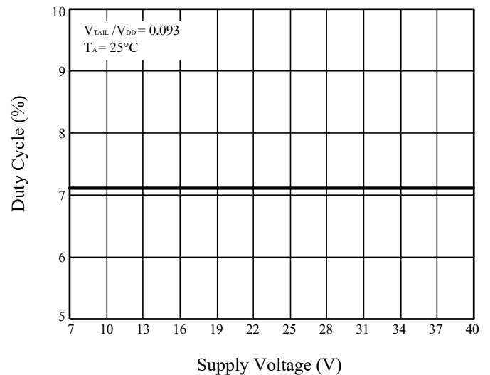
Figure 14 Duty Cycle vs. Supply Voltage (Internal PWM)
