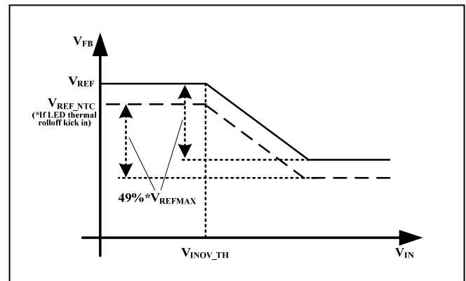
Figure 37 VIN Over Voltage Protection
