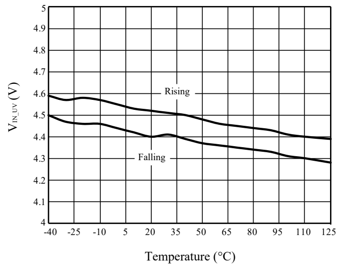
Figure 20 V_{IN\_UV} vs. Temperature
