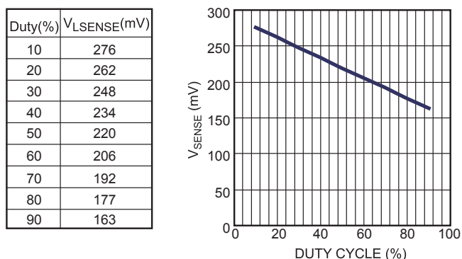
Figure 2: V_{SENSE} vs Duty Cycle
