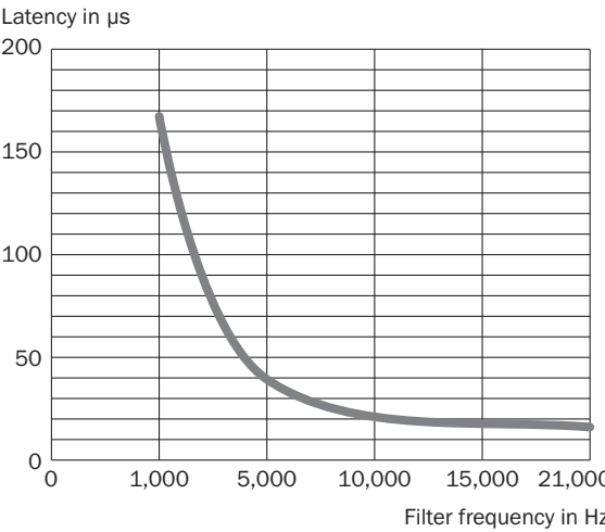
This diagram shows the switch-on current Latency vs. filter frequency
