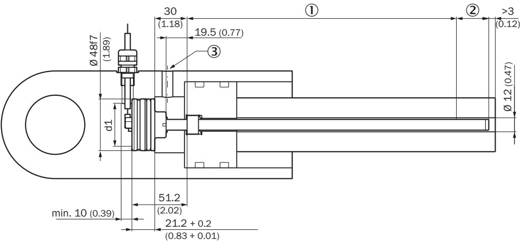
Installation space for cylinders
