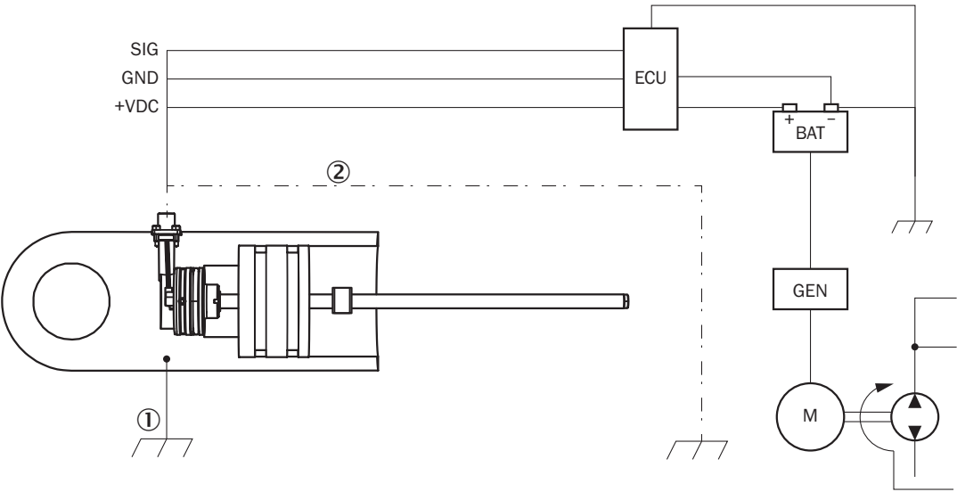
Connection diagram
