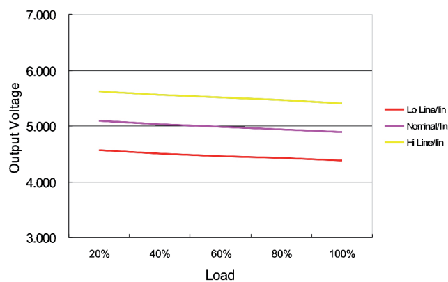
1S7BE_12yy type
