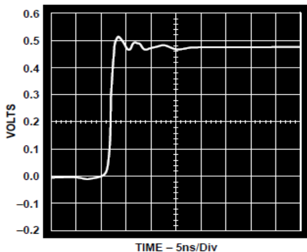
Figure 11. Step Response
