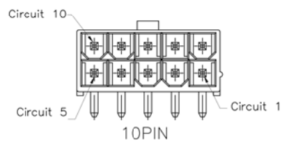
2~24P Protection Key Drawing(Ref.)
