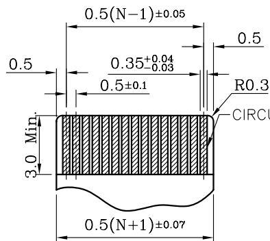
RECOMMENDED APPLICABLE FPC LAYOUT (THICKNESS:0.3±0.03)
