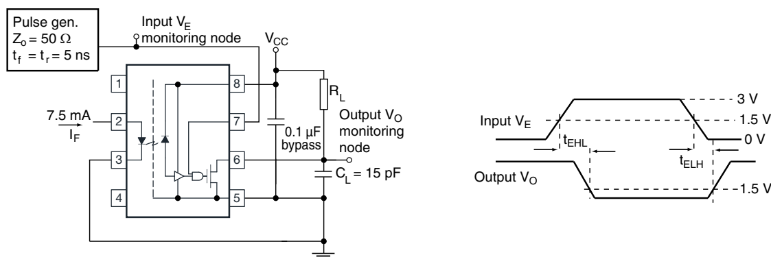
Fig. 3 - Test Circuit for t_{EHL} and t_{ELH}
