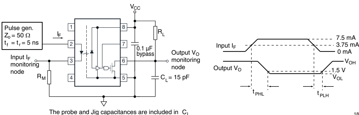
Fig. 2 - Test Circuit for t_{PLH} , t_{PHL} , t_r , and t_f
