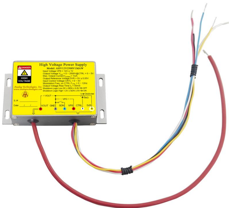
Figure 1.1. Top View of AHV12V2500V1MAW
