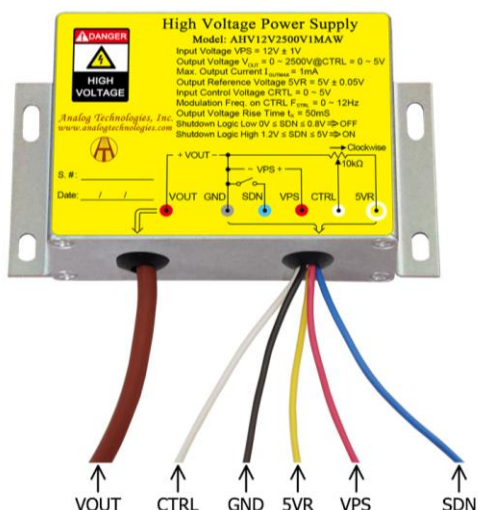
Figure 2. The Connecting Lead Wires of AHV12V2500V1MAW
