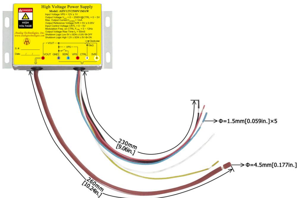
Figure 13. Connecting Lead Wires of AHV12V2500V1MAW
