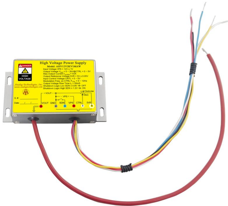
Figure 1.1. Top View of AHV12V2KV1MAW
