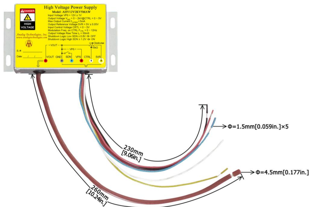
Figure 13. Connecting Lead Wires of AHV12V2KV5MAW
