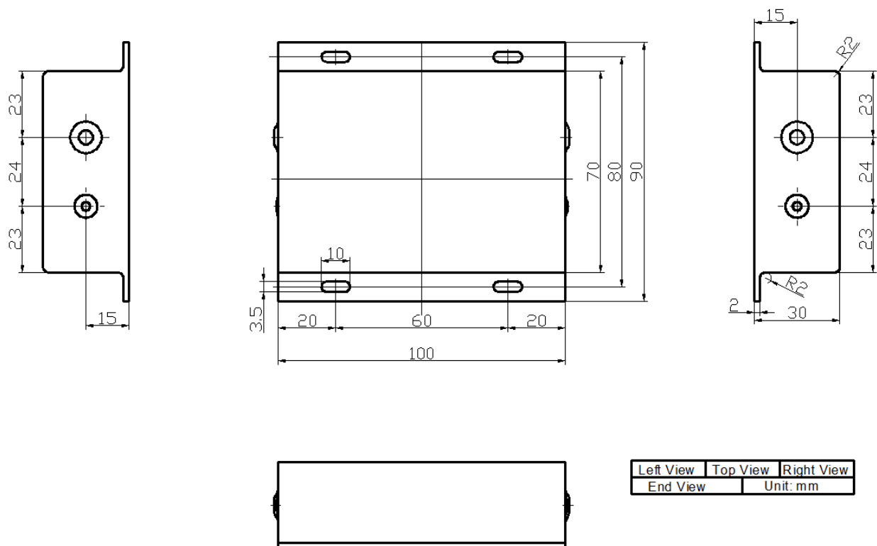
Figure 13. Outline Dimensions
