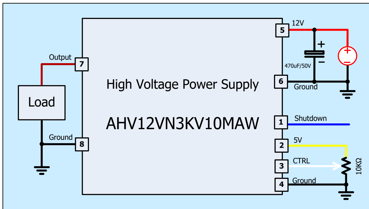
Figure 2. Setting Output to be a Constant Voltage
