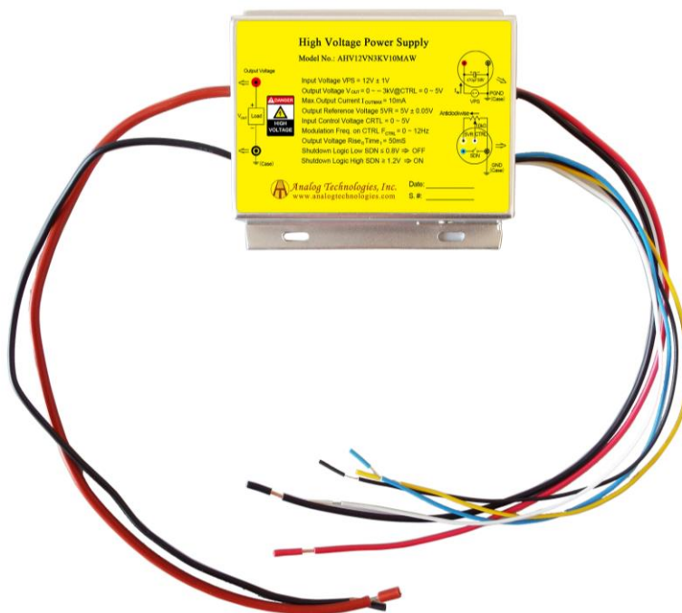
Figure 12. Connecting Lead Wires of AHV12VN3KV10MAW
