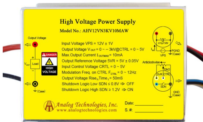
Figure 1. Physical Photo of AHV12VN3KV10MAW
