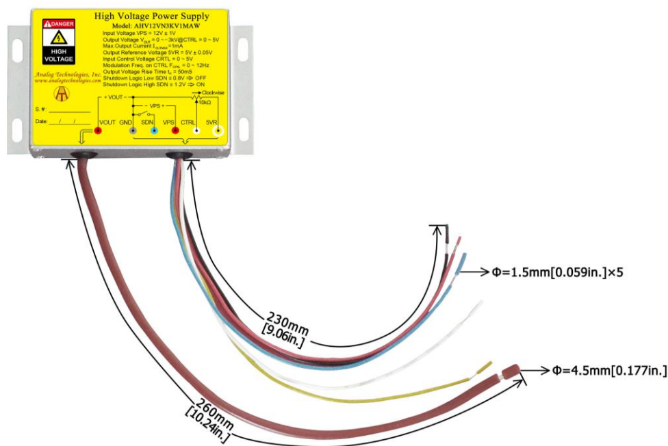
Figure 13. Connecting Lead Wires of AHV12VN3KV1MAW
