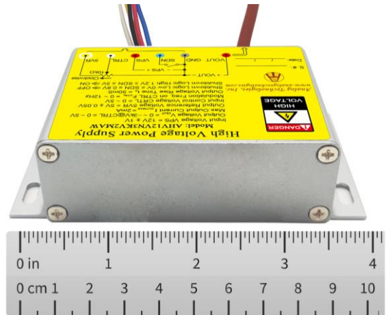
Figure 1.3. Side View
