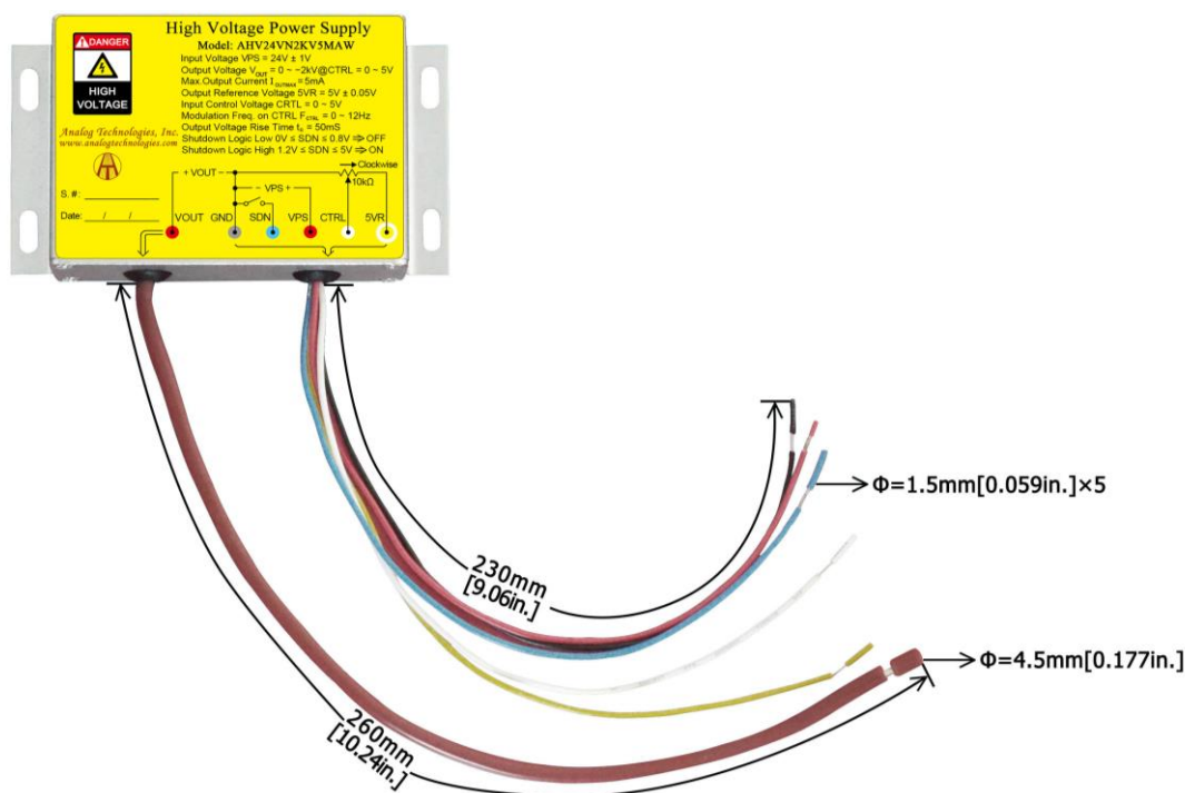
Figure 13. Connecting Lead Wires of AHV24VN2KV5MAW
