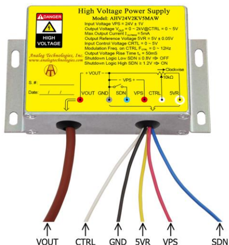
Figure 2. The Connecting Lead Wires of AHV24V2KV5MAW
