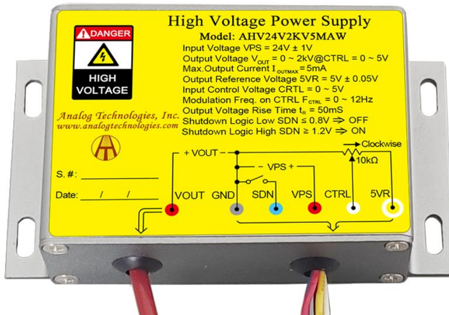
Figure 1.1. Top View of AHV24V2KV5MAW
