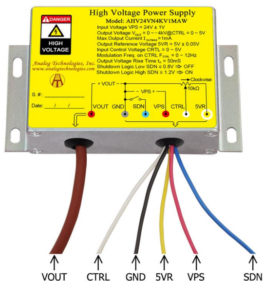
Figure 2. The Connecting Lead Wires of AHV24VN4KV1MAW
