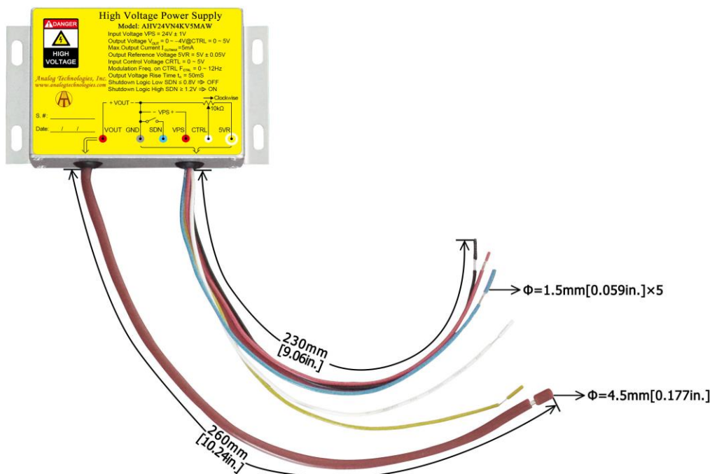
Figure 13. Connecting Lead Wires of AHV24VN4KV5MAW
