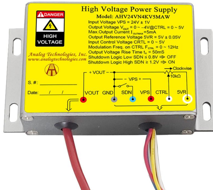
Figure 1.1. Top View of AHV24VN4KV5MAW
