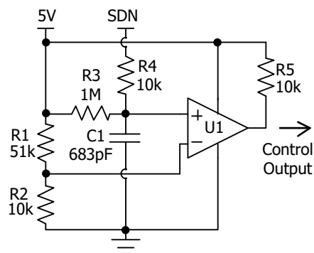
Figure 6. The Equivalent Circuit for SDN Port
