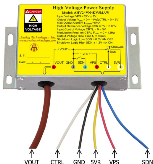
Figure 2. The Connecting Lead Wires of AHV24VN4KV5MAW
