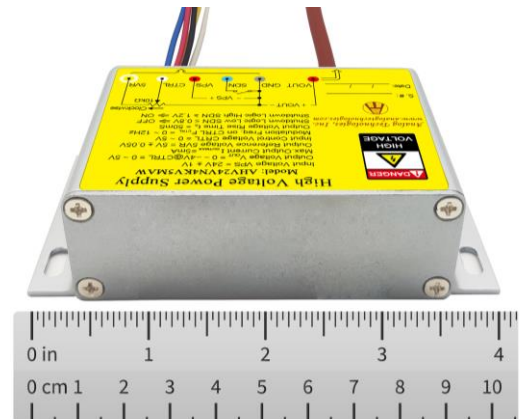
Figure 1.3. Side View
