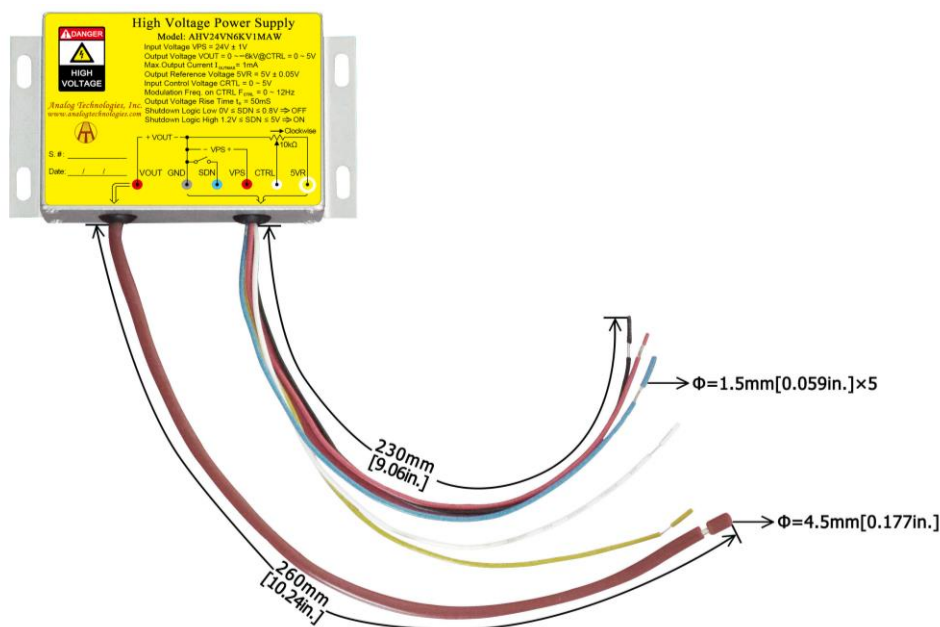
Figure 13. Connecting Lead Wires of AHV24VN6KV1MAW
