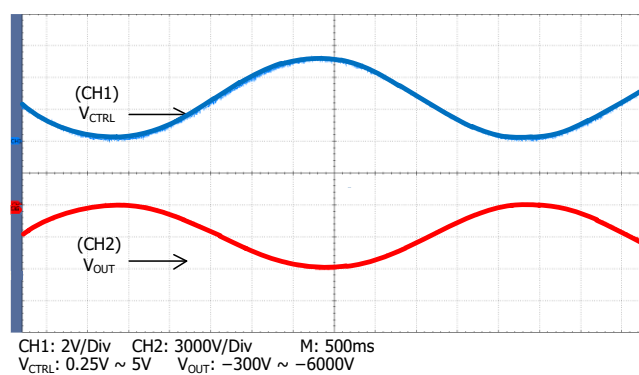
Figure 9. Sine Wave Modulation
