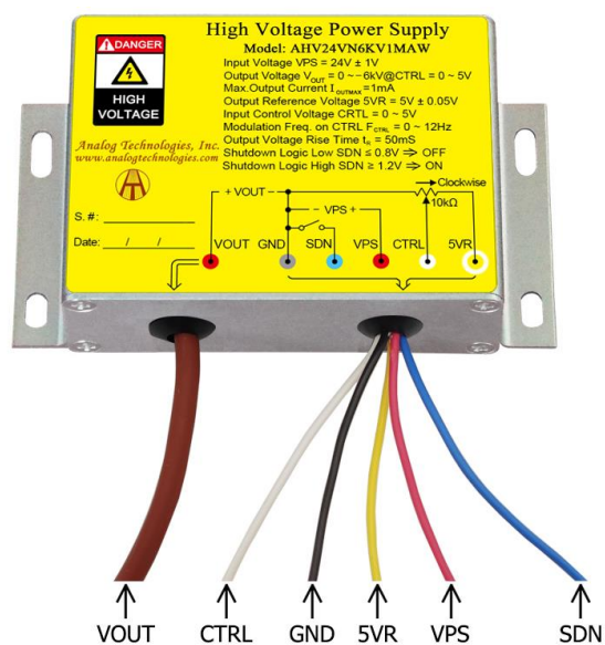
Figure 2. The Connecting Lead Wires of AHV24VN6KV1MAW
