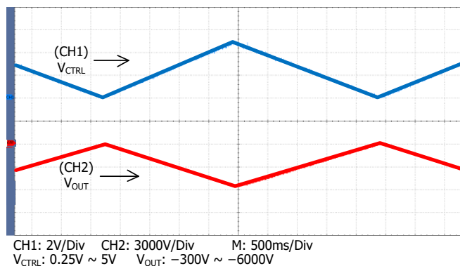
Figure 8. Triangle Wave Modulation
