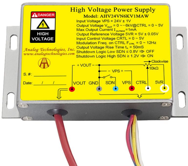
Figure 1.1. Top View of AHV24VN6KV1MAW
