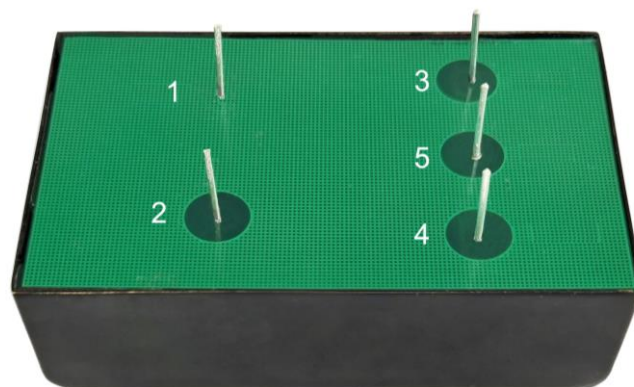
Figure 1. Physical Photos of AHVR12V1KV10MAP
