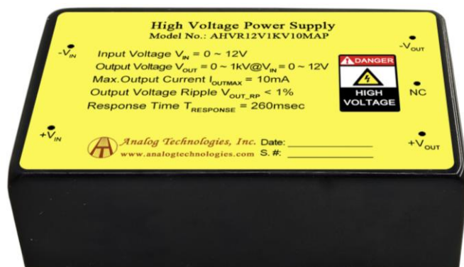
Figure 1. Physical Photos of AHVR12V1KV10MAP
