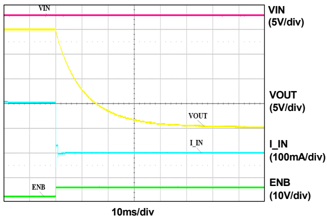
Figure 7. Shutdown (VIN=20V)
