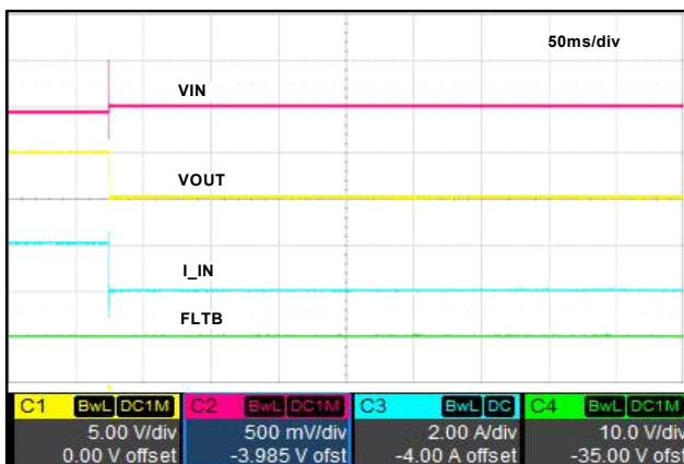
Figure 17. Short Circuit Protection (LOAD = 2.5Ω, Device Option -04)
