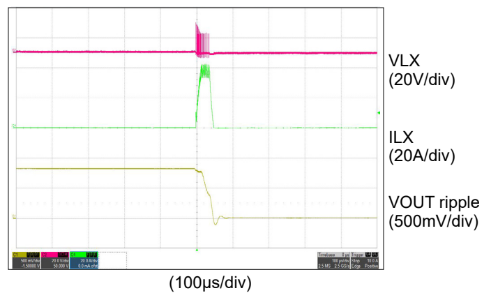
Short-Circuit Protection
