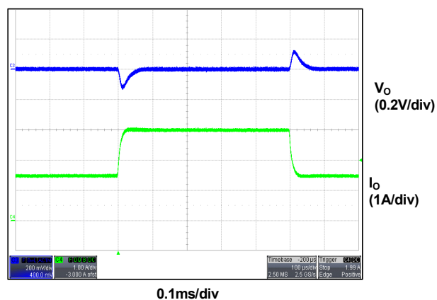
Figure 9. 50% to 100% Load Transient
