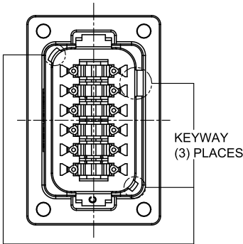
P/N AT04-12PC-PM02 KEY-C CONFIGURATION STANDARD COLOR: GREEN
