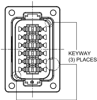
P/N AT04-12PD-PM02 KEY-D CONFIGURATION STANDARD COLOR: BROWN
