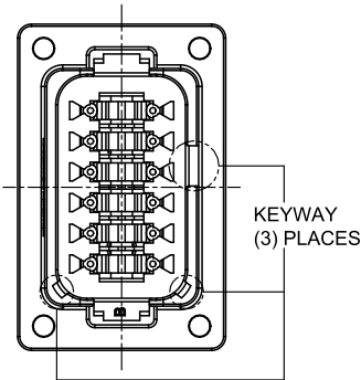
P/N AT04-12PB-PM02 KEY-B CONFIGURATION STANDARD COLOR: BLACK
