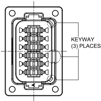
P/N AT04-12PA-PM02 KEY-A CONFIGURATION STANDARD COLOR: GREY
