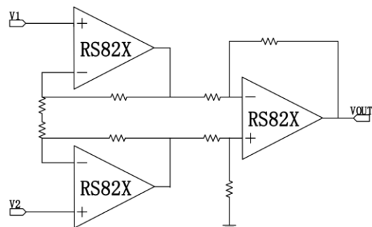
Figure 3. Amplifier Instrumentation Amplifier
