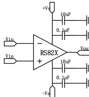
Figure 2. Amplifier with Bypass Capacitors
