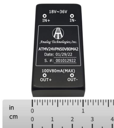
Figure 1. Top View of ATMV24VPN50V80MA2
