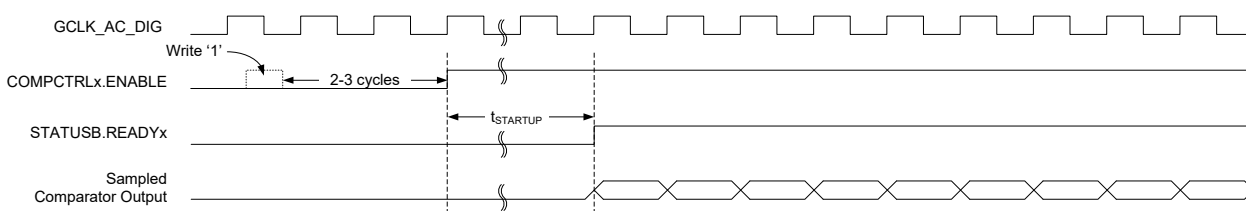
Figure 29-2. Continuous Measurement Example
