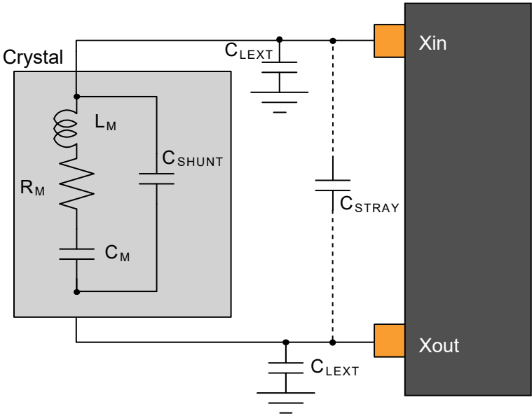
Figure 33-4. Oscillator Connection
