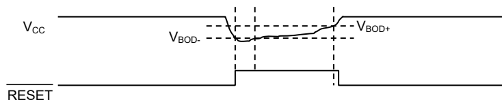
Figure 32-4. BOD33 Hysteresis ON
