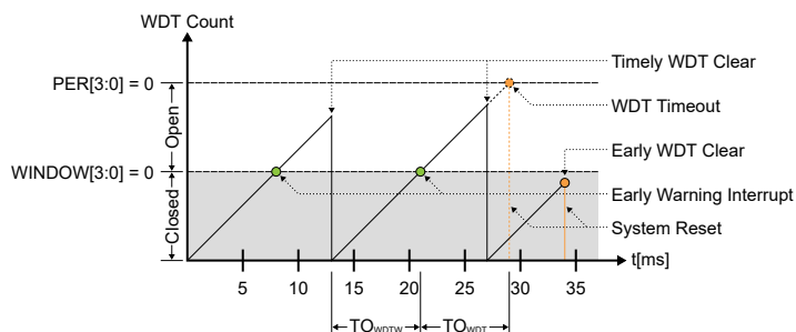
Figure 17-3. Window-Mode Operation
