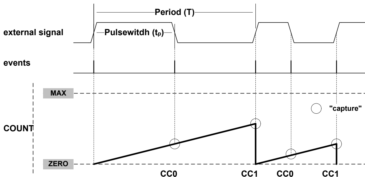
Figure 27-10. PWP Capture
