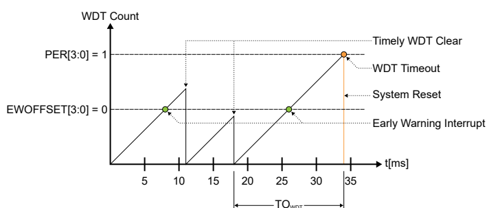
Figure 17-2. Normal-Mode Operation
