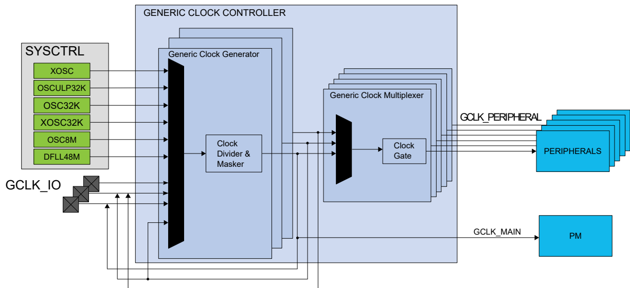
Figure 14-1. Device Clocking Diagram
