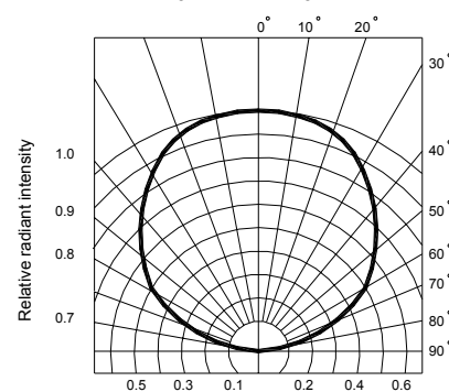
Fig.6 Radiation diagram
