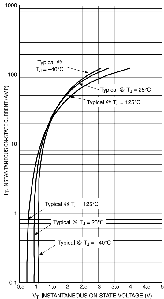
Figure 3. On-State Characteristics
